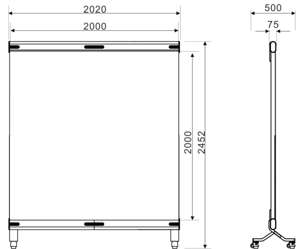
▼ External dimensions:2000*2000mm
