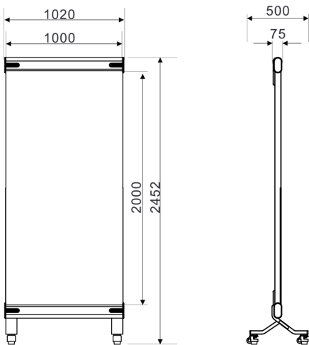
▼ External dimensions:1000*2000mm
